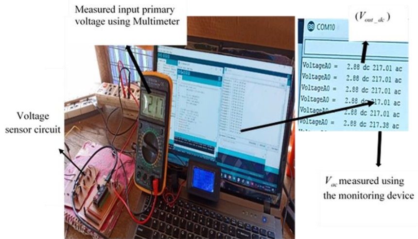
FIGURE 3. Experimental setup for voltage calibration
