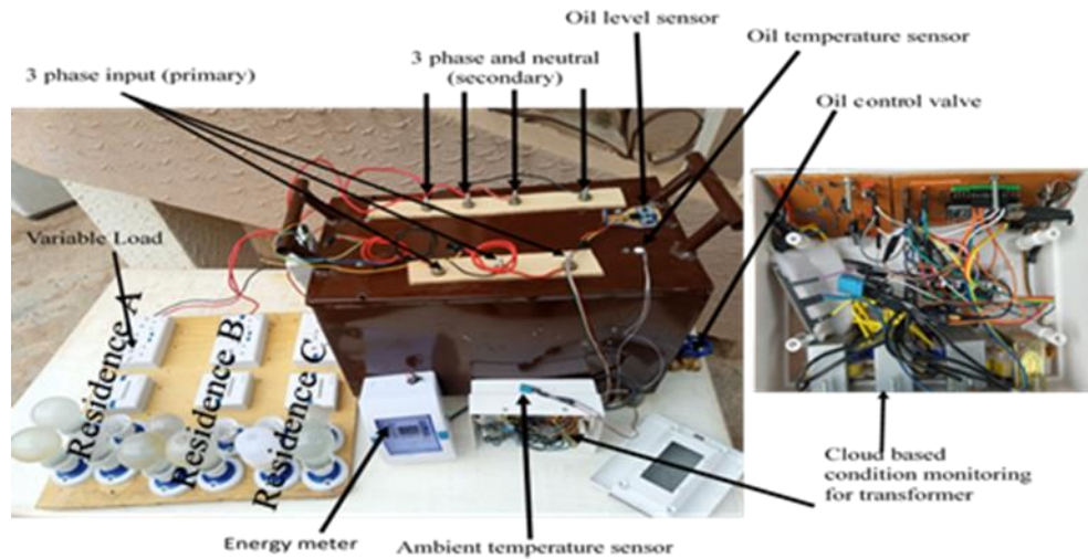
FIGURE 11. Experimental setup for cloud-based condition monitoring device
