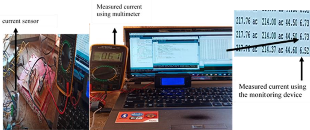
FIGURE 4. Experimental setup for current calibration
