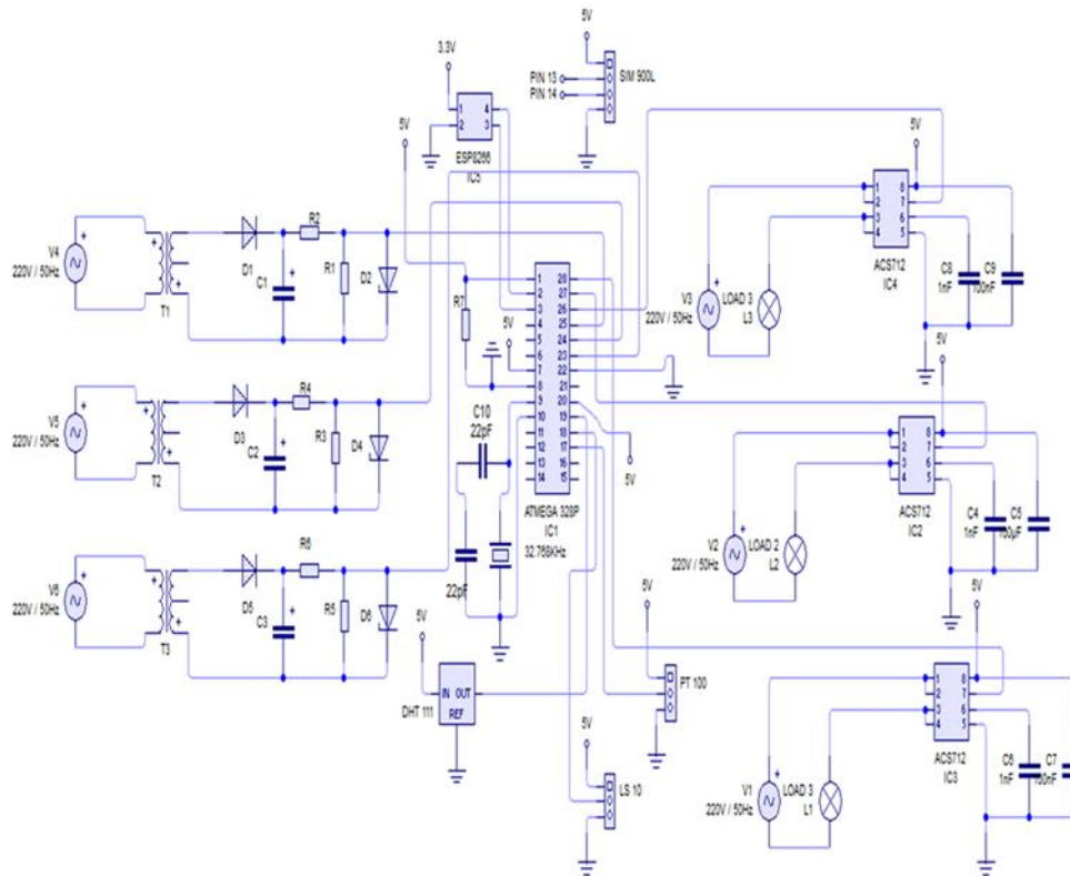
FIGURE 10. Circuit diagram of the monitoring device
