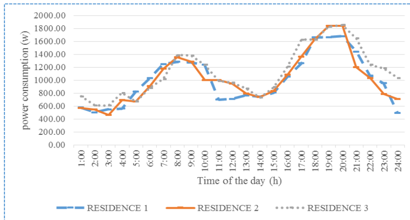
FIGURE 17. Average weekdays power consumed by the consumer in the residents for 24 hours load cycle
