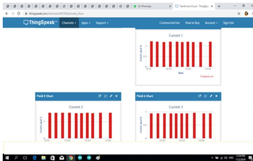
FIGURE 14. Real-time monitoring of the three-phase current of the distribution transformer on the thingSpeak server
