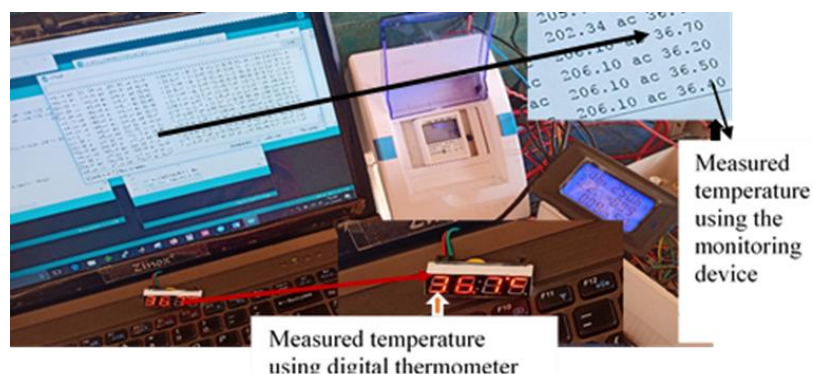
FIGURE 5. Experimental setup for temperature calibration
