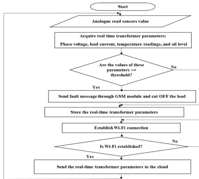
FIGURE 9. Algorithm flow chart for the monitoring device
