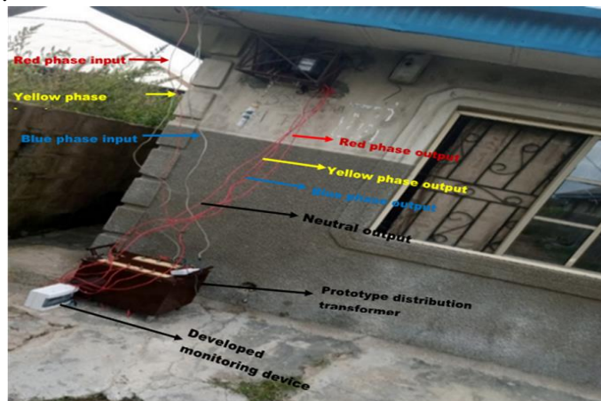
FIGURE 12. Wiring connection of the device to the residences
