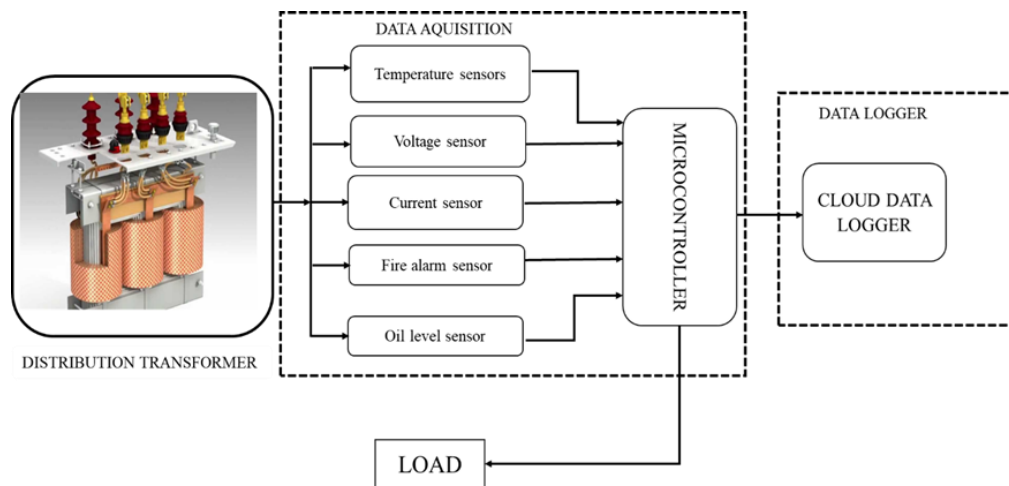
FIGURE 1. Cloud-based condition monitoring of distribution transformer
